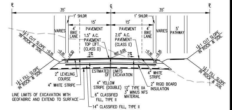
TYPICAL SECTION – Collector Road
